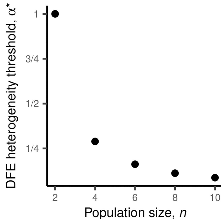
Fig 2. DFE heterogeneity required to justify maximal diversification. The \alpha^* at which it becomes more advantageous to diversify maximally than to not diversify at all in our two-parent model (where the DFE rate parameters \lambda are distributed as \text{Exponential}(\alpha) ). Note that, for small n , the DFE heterogeneity \alpha must be roughly on the order of the fitness difference between parents \Delta x to justify maximum diversification. However, as n increases, maximal diversification can be favorable even when \alpha is substantially less than \Delta x .
