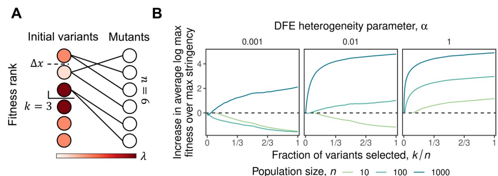
Fig 3. The effect of selection stringency in the k -parent model. (A) Schematic of the k -parent model, here with n = 6 and k = 3 . (B) Simulations of the k -parent model (with \Delta x = 1 ) showing how the maximum fitness of the mutants depends on the selection stringency, i.e. the fraction of variants selected as parents for the next round, k/n . Note that the advantage of diversification increases with n and with the degree of heterogeneity between the DFEs of the parents.
