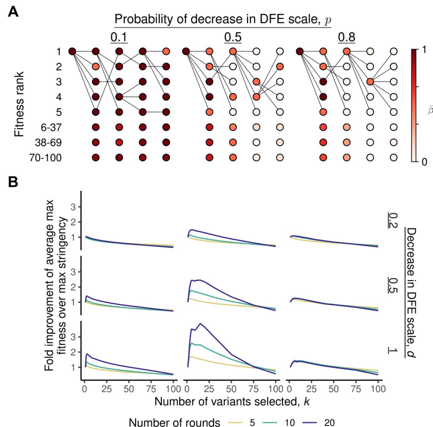
Fig 4. Effects of selection stringency in the k -parent inheritance model. (A) Examples of the dynamics across four rounds of directed evolution in our k -parent inheritance model for three different probabilities p of DFE degradation. Here d = 0.5 , n = 100 , and the selection stringency is k = 5 . For variants not among the fittest k , color reflects the average \beta in that bin. Edges indicate parentage, though edges to variants below the top k are not shown. (B) At a population size of n = 100 , the average maximum fitness at the end of 5, 10, and 20 rounds of directed evolution as a function of selection stringency k and the features of DFE inheritance ( p and d ).
