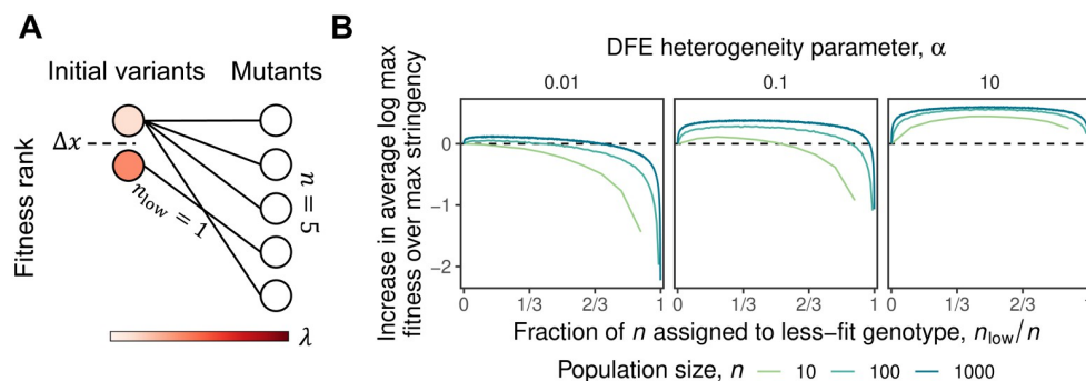
Fig 1. The immediate effect of selection stringency on fitness while drawing mutants from two parents. (A) Schematic of our two-parent model, in which we assume that we generate mutants for the next round (here a total of n = 5 mutants) from two parental variants of different fitness. In this model, the selection stringency is determined by the number of mutants we draw from the lower-fitness parent, which has a fitness disadvantage of \Delta x compared to the higher-fitness parent. We assume that each parent has an exponential DFE, with parameter \lambda that is drawn at random as described in the text. (B) Simulations of the two-parent model (with \Delta x = 1 ) showing how the maximum fitness of the mutants depends on the selection stringency, i.e. the fraction of the mutants drawn from the less-fit parent. Note that the advantage of diversification increases with n and with the degree of heterogeneity between the DFEs of the parents.
