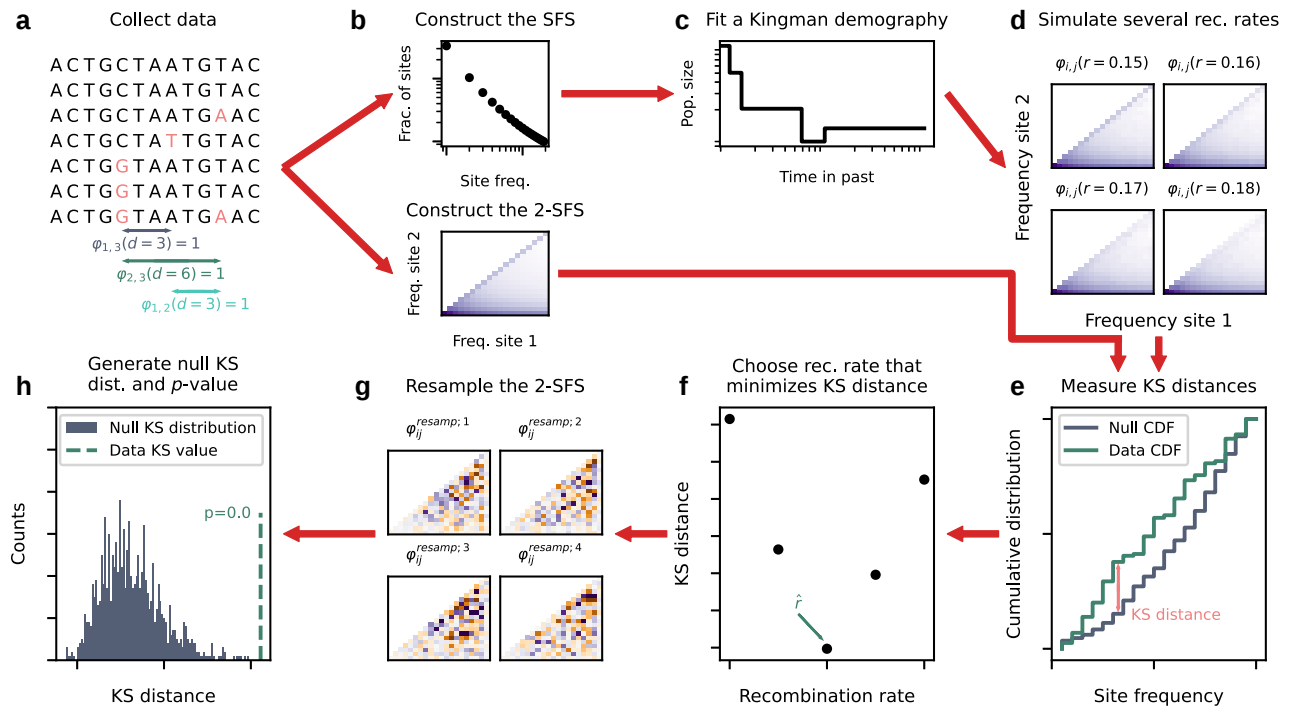
Fig. 1. Schematic of the model-checking pipeline. The pipeline follows the arrows from a to h. Briefly, after data collection and cleaning a), we construct the SFS and 2-SFS b) and fit a Kingman demography (the null model) to the SFS c). We simulate the 2-SFS expected from a Kingman model with this null demography for several values of the recombination rate, \hat{r} , that maximizes the P-value for rejecting the Kingman model based on the KS distance between the 2-SFS of the data and the null d–f). We then resample \phi_{ij}^{null}(d; \hat{r}) g) and compute the KS distance between these resampled distributions and \phi_{ij}^{null}(d; \hat{r}) to generate a null KS distribution. We compare the KS distance between \phi_{ij}^{data}(d) and \phi_{ij}^{null}(d; \hat{r}) to this null KS distribution to generate a P-value h).
